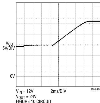
Soft Start-Up
