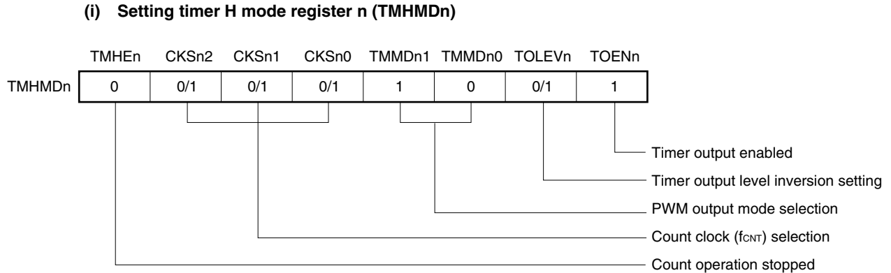
Figure 8-11. Register Setting in PWM Output Mode
