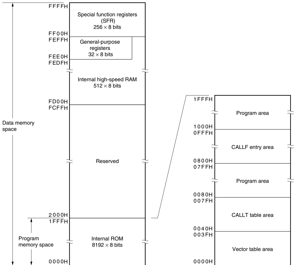
Figure 3-1. Memory Map ( \mu PD780121)
