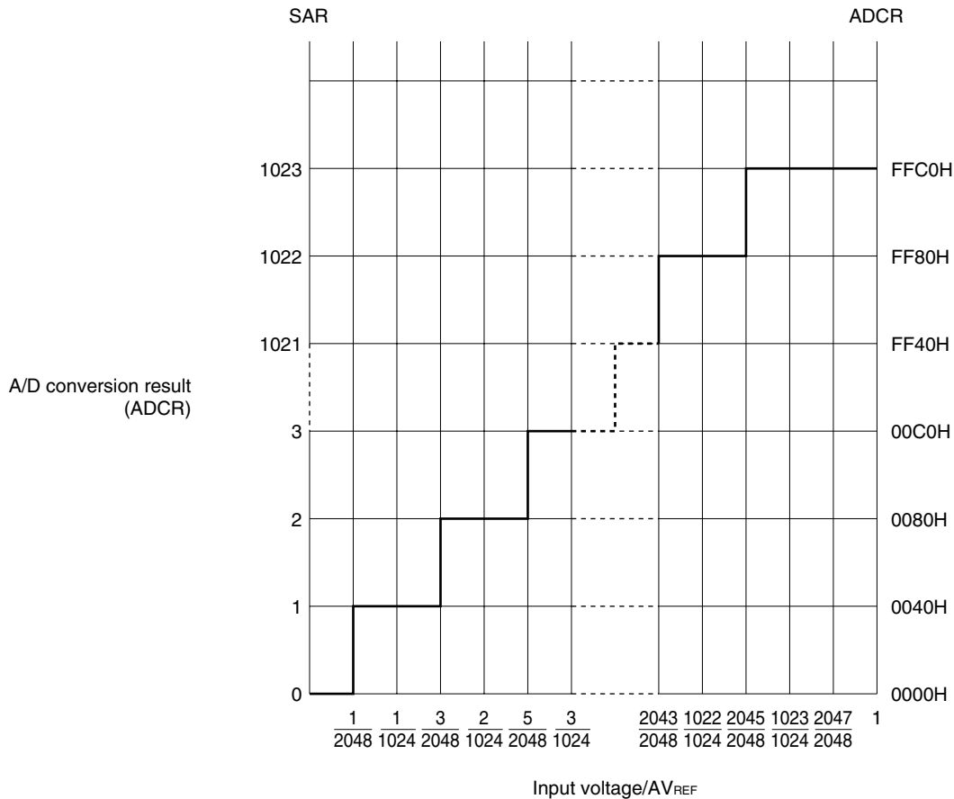
\star Figure 12-9. Relationship Between Analog Input Voltage and A/D Conversion Result
