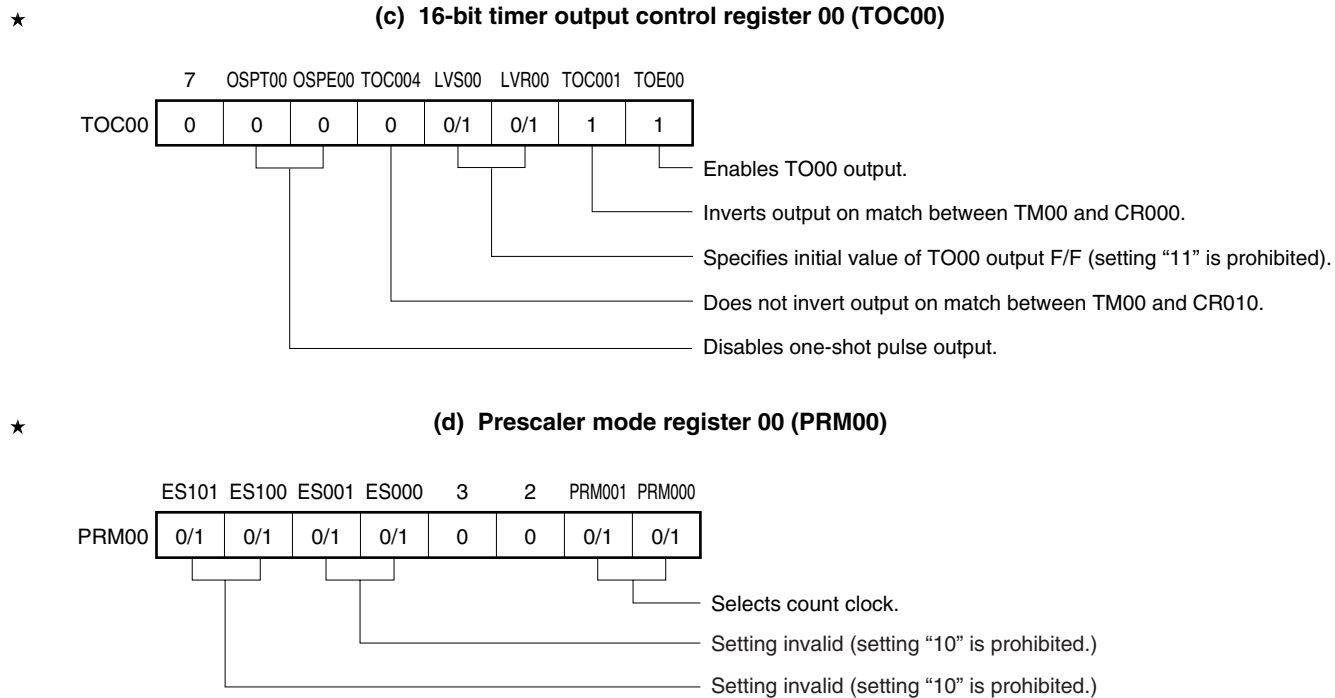
Figure 6-29. Control Register Settings in Square-Wave Output Mode (2/2)
