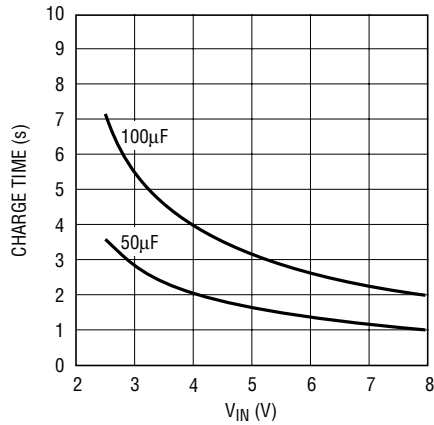
LT3484-0 Charge Time
