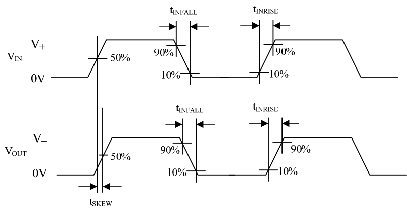
Test Circuit 4. Output Signal Skew
