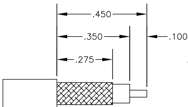
STRIPPING DIMENSIONS
