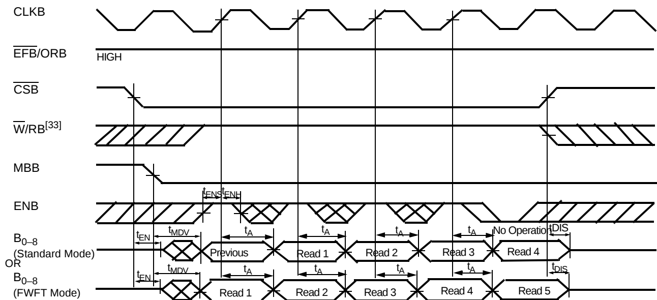
Port B Byte Read Cycle Timing for FIFO1 (CY Standard and FWFT Modes) [1, 36]
