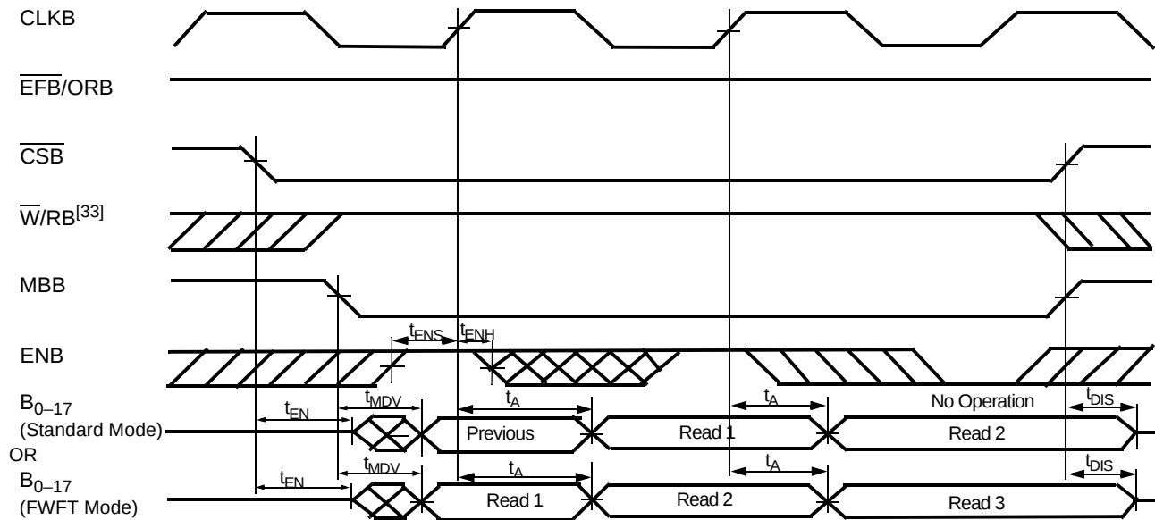
Port B Word Read Cycle Timing for FIFO1 (CY Standard and FWFT Modes) [1, 37]
