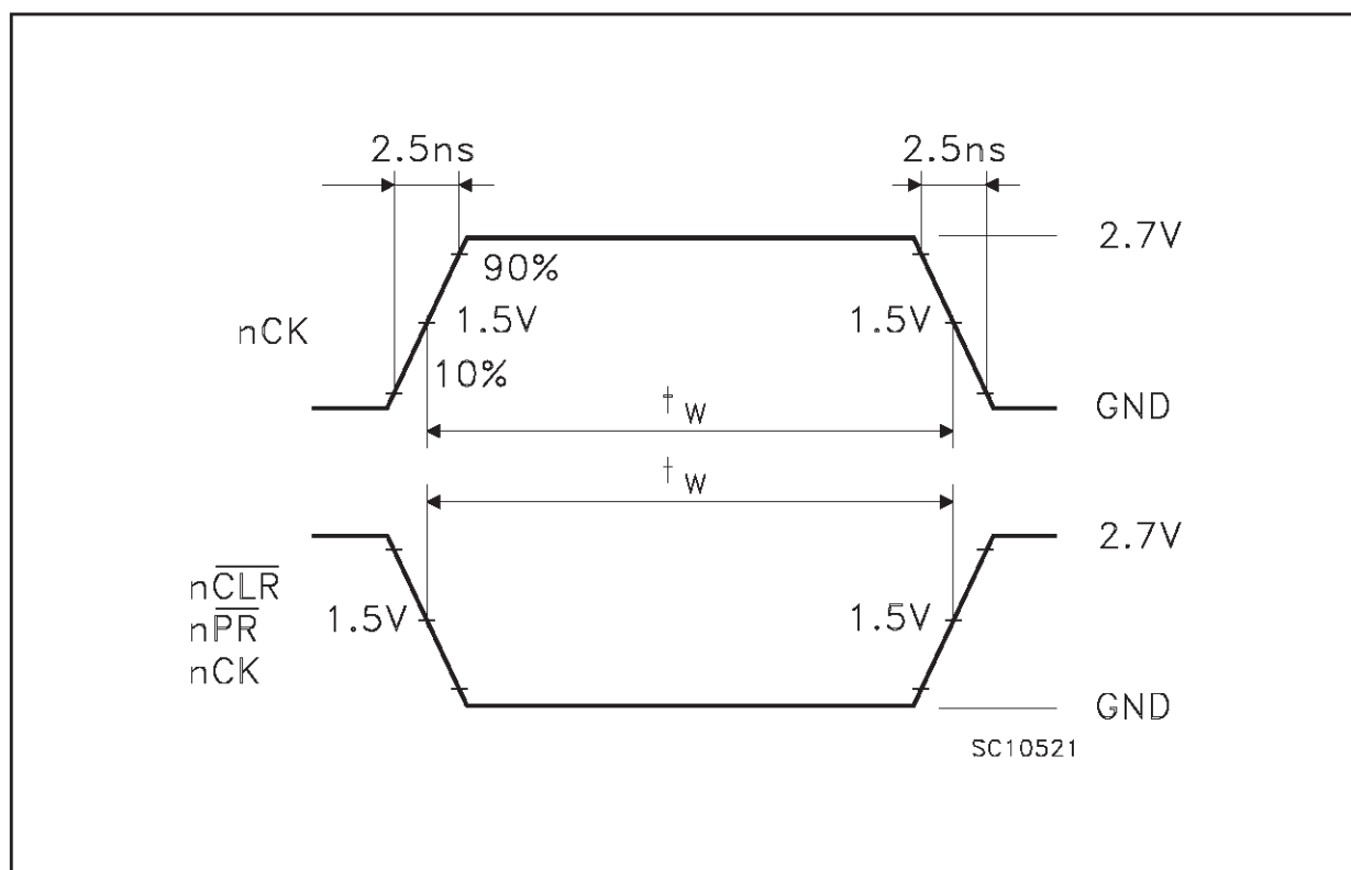
WAVEFORM 4 : PULSE WIDTH ( f=1\text{MHz} ; 50% duty cycle)
