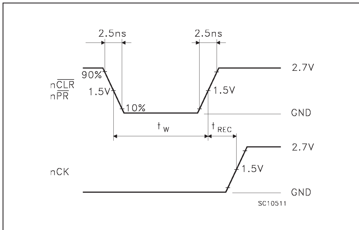
WAVEFORM 3 : RECOVERY TIMES ( f=1\text{MHz} ; 50% duty cycle)
