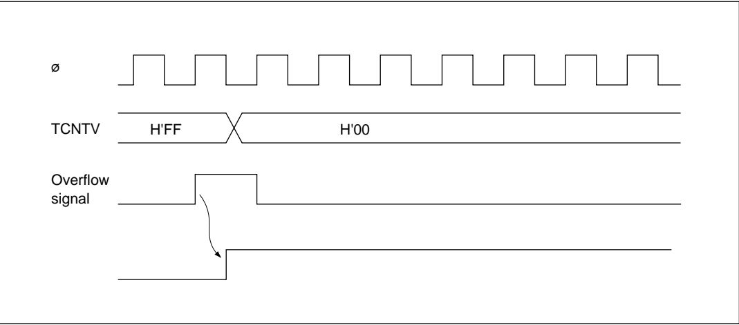
Figure 9-6 OVF Set Timing
