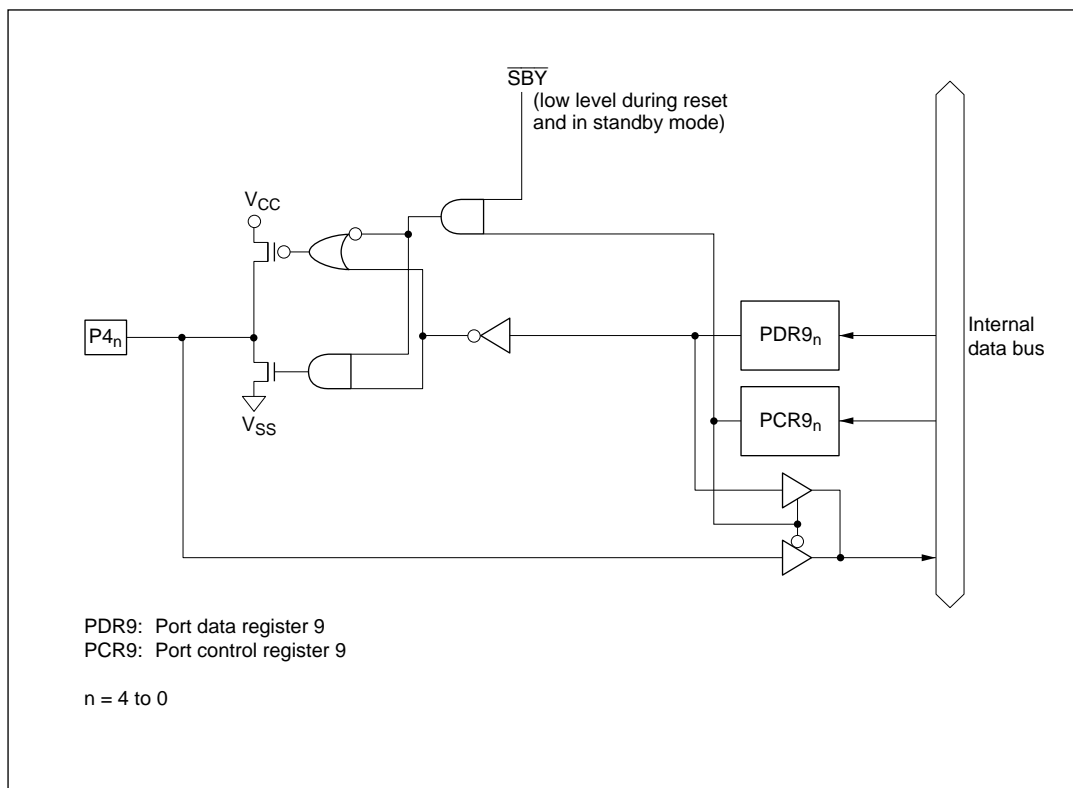
Figure C-8 Port 9 Block Diagram (Pins P9_7 to P9_3 )
