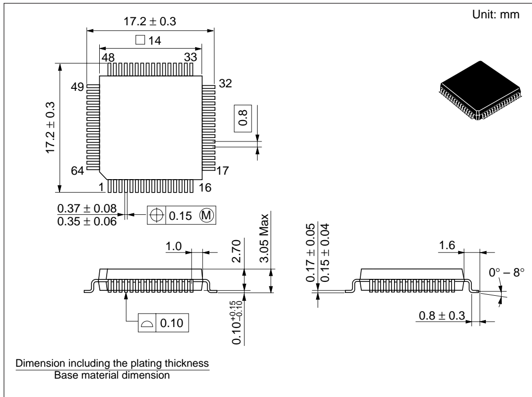
Figure F-1 FP-64A Package Dimensions
