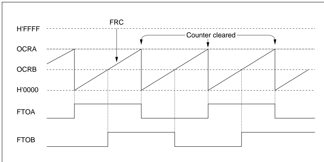
Figure 9-31 Pulse Output Example
