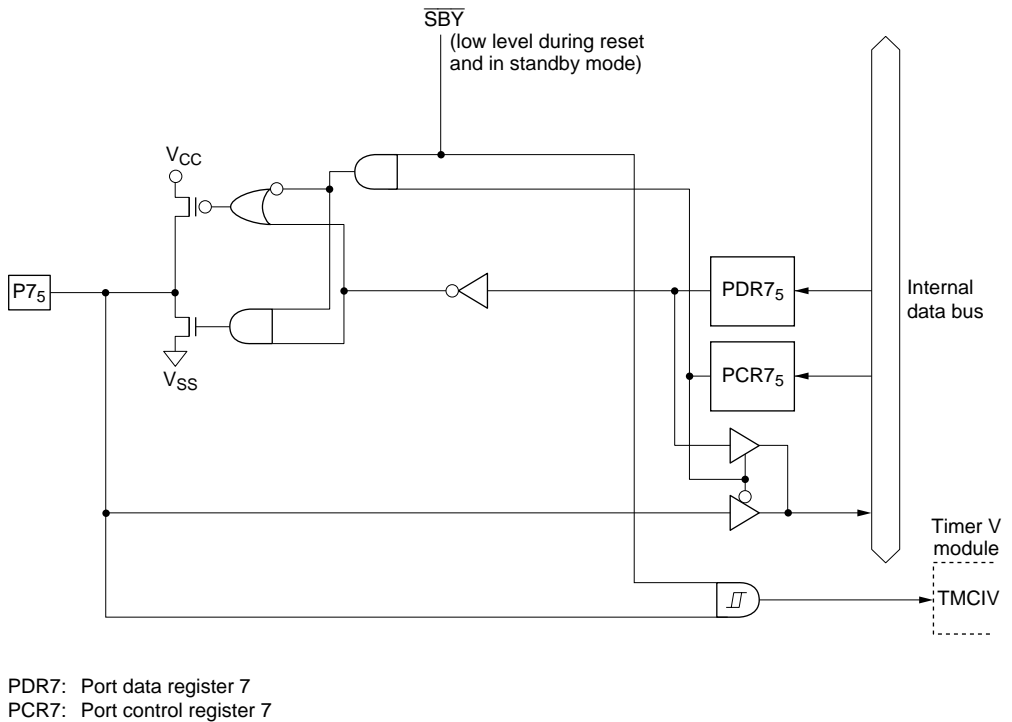
Figure C-6 (c) Port 7 Block Diagram (Pin P7 5 )
