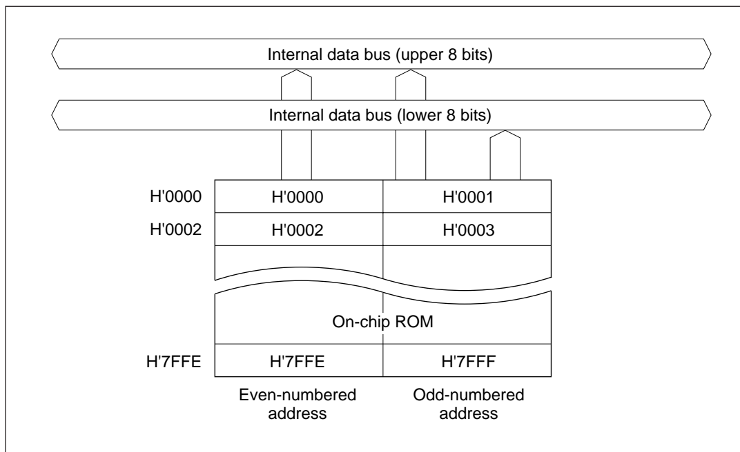
Figure 6-1 ROM Block Diagram (H8/3644)
