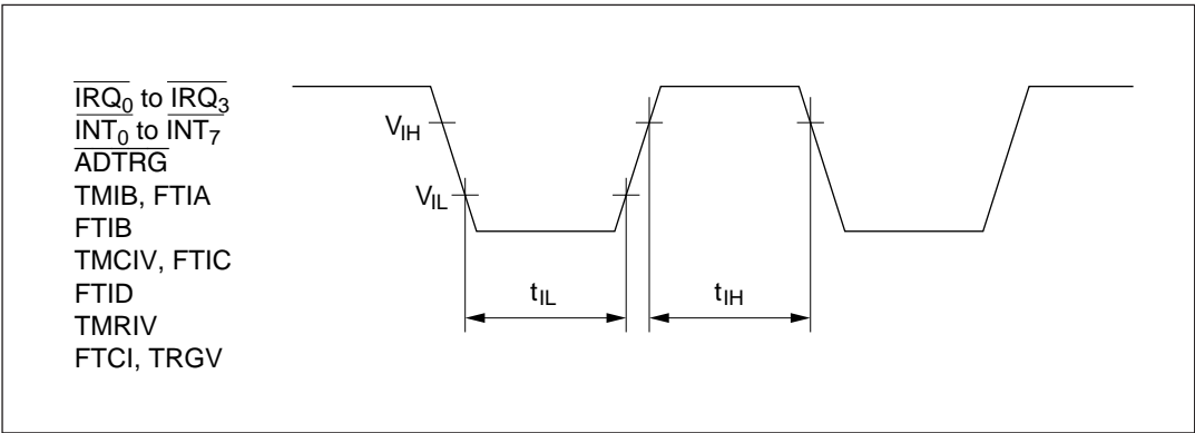
Figure 13-3 Input Timing
