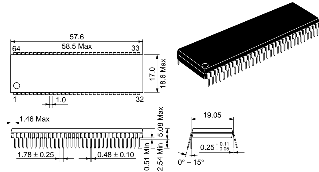
Figure F-2 DP-64S Package Dimensions
