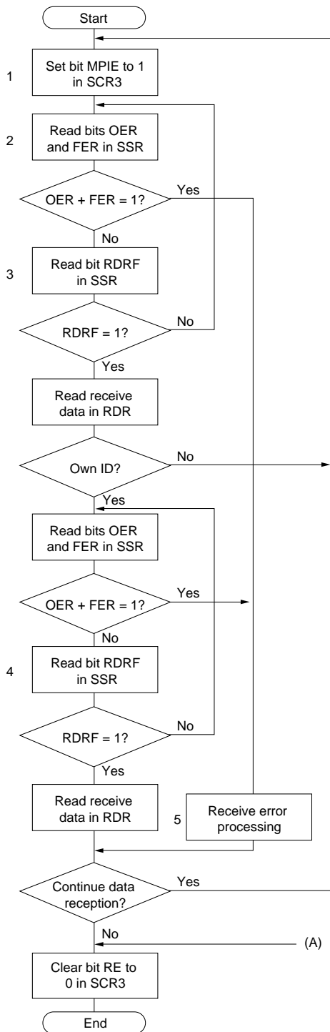
Figure 10-24 Example of Multiprocessor Data Reception Flowchart
