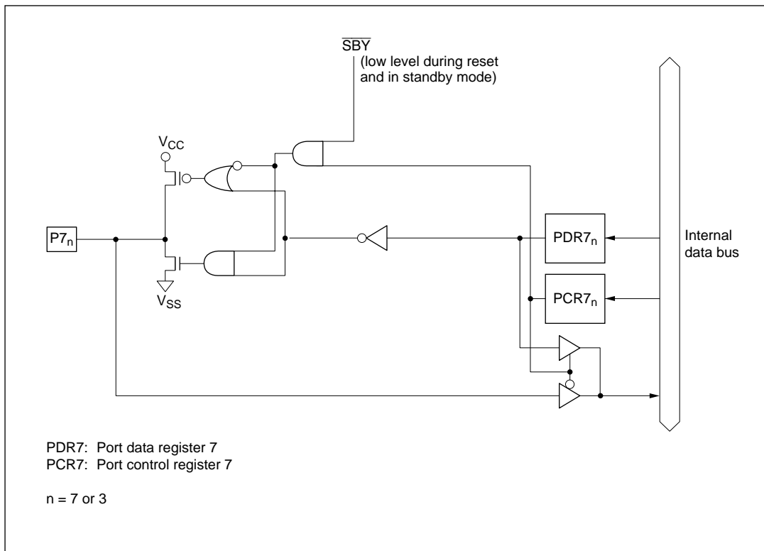
Figure C-6 (a) Port 7 Block Diagram (Pins P7 7 and P7 3 )
