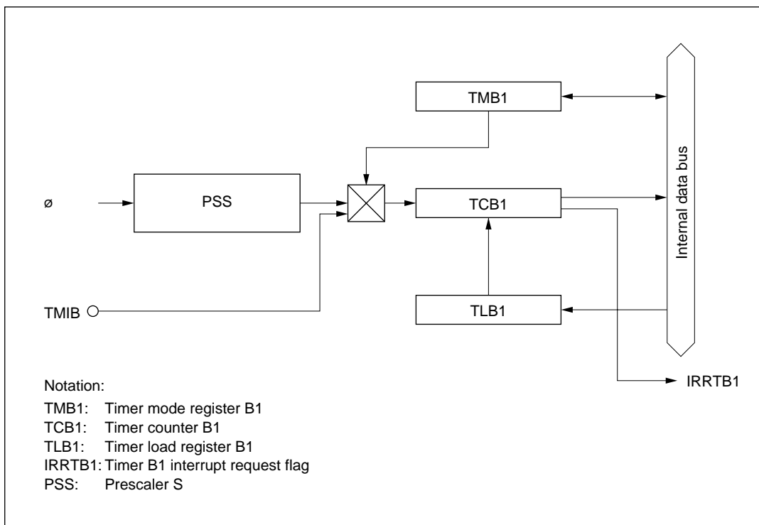
Figure 9-2 Block Diagram of Timer B1
