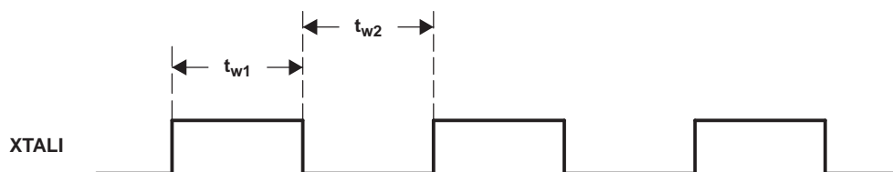
Figure 10. Clock Input
