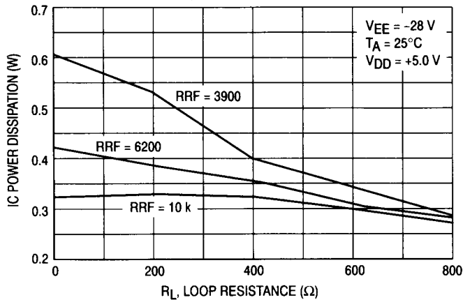
Figure 23. IC Power Dissipation versus Loop Resistance and RRF
