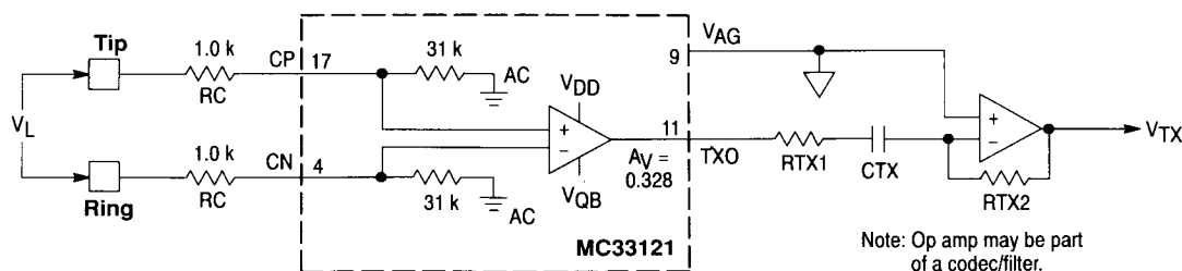
Figure 28. Transmit Path
