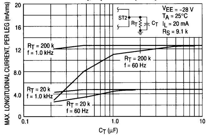
Figure 26. Maximum Longitudinal Current versus CT, RT and Frequency
