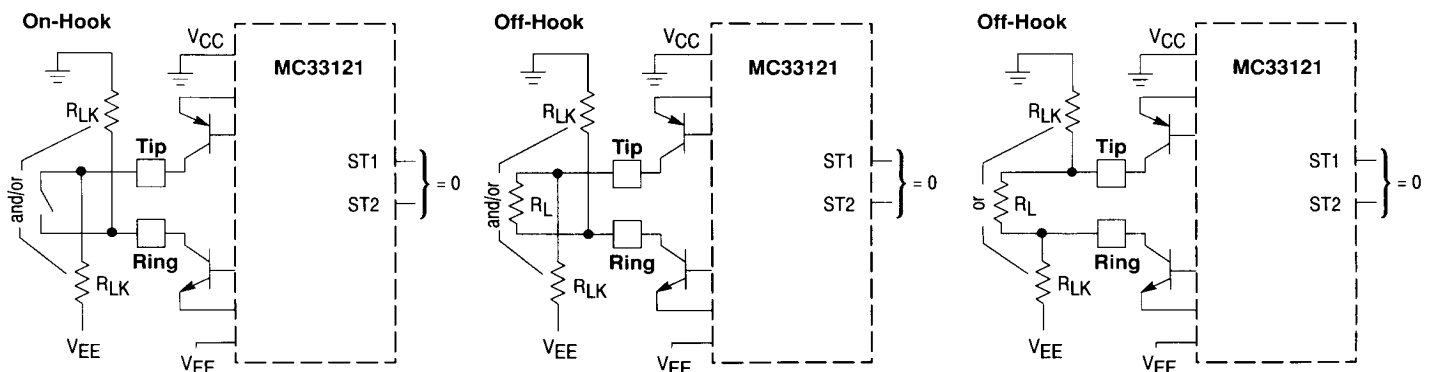
Figure 38. Fault Detection
