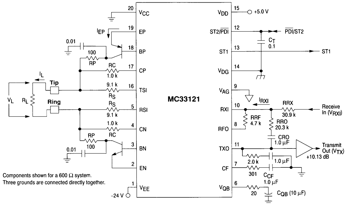
Figure 1. Test Circuit
