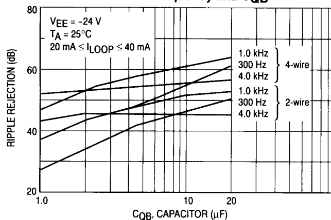
Figure 18. VEE Ripple Rejection versus Frequency and CQB
