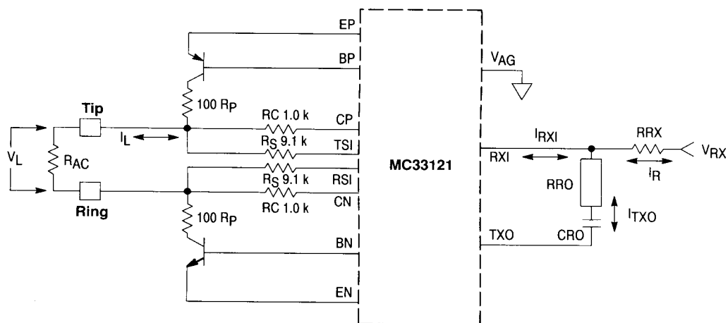
Figure 35. Receive Gain
