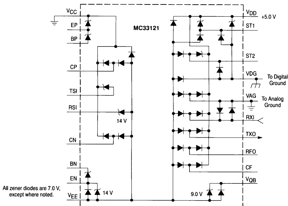
Figure 40. Protection Diodes
