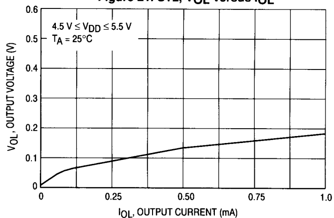
Figure 21. ST2, VOL versus IOL
