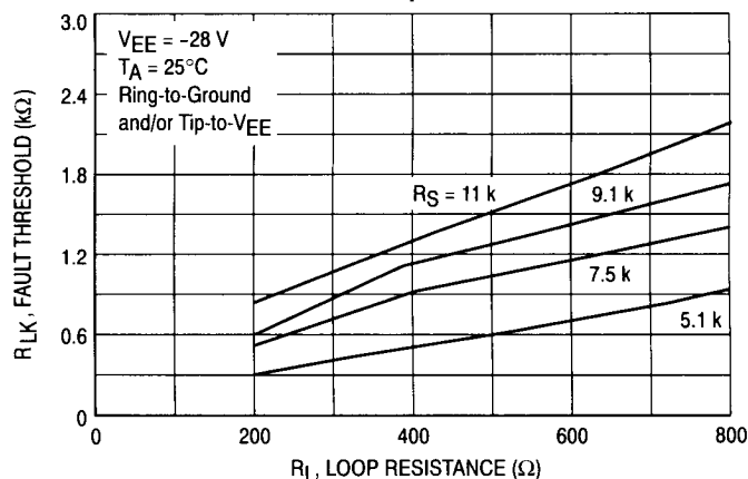
Figure 13. Fault Threshold (Off-Hook) versus Loop Resistance
