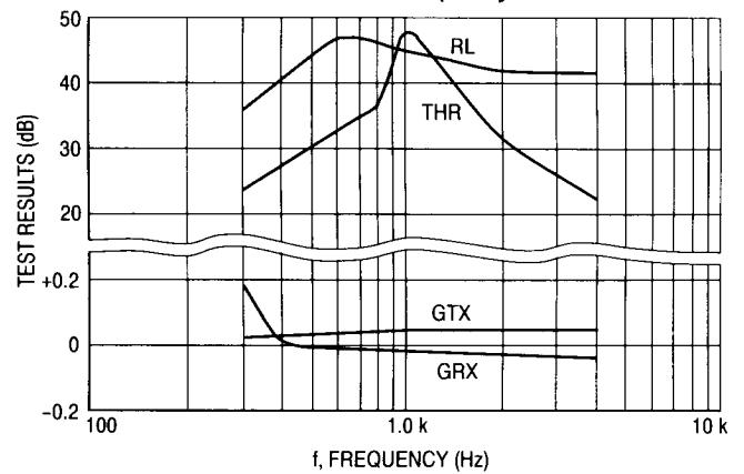
Figure 50. Circuit Performance 900 \Omega and 2.16 \mu F System
