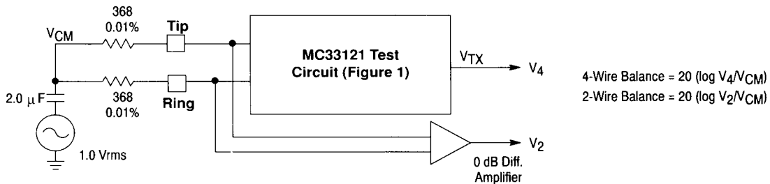
Figure 2. Longitudinal Balance Test
