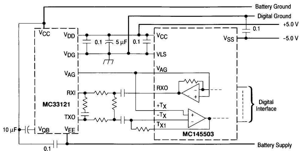
Figure 42. Connection to a CODEC With Separate Grounds
