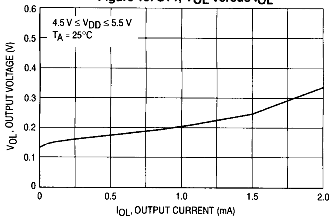
Figure 19. ST1, VOL versus IOL
