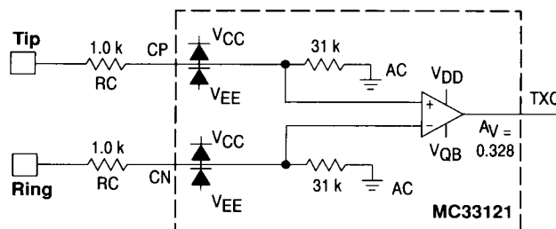
Figure 32. RC Protection Resistors
