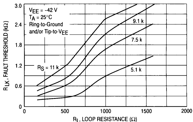
Figure 12. Fault Threshold (Off-Hook) versus Loop Resistance
