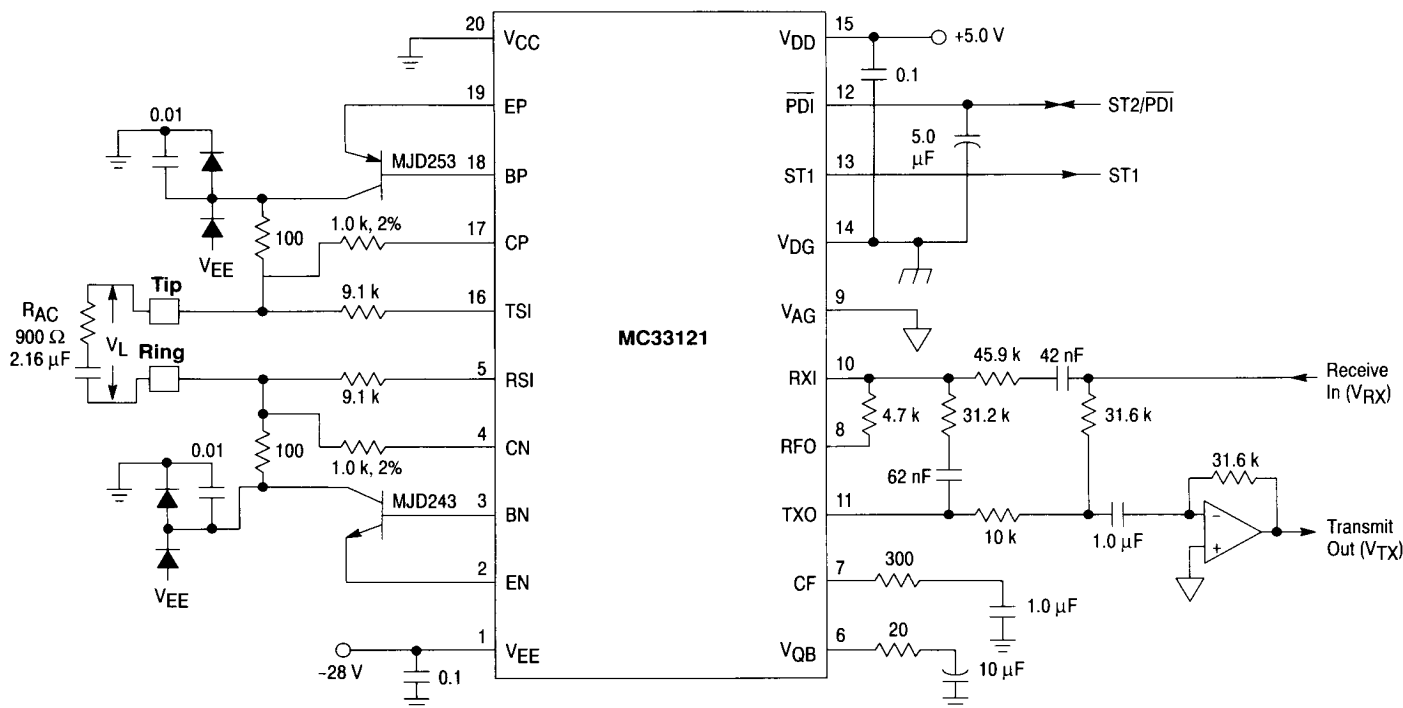
Figure 47. 900 \Omega and 2.16 \mu\text{F} System
