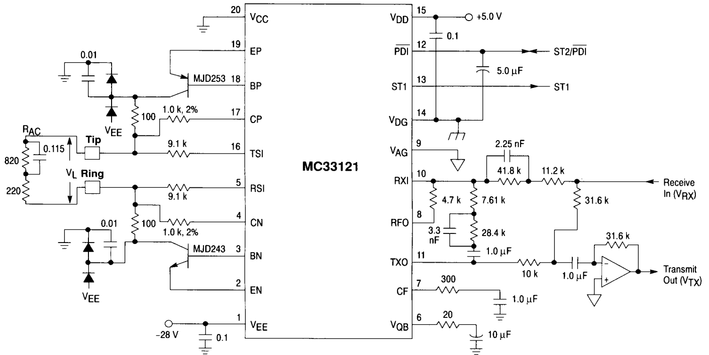
Figure 48. 220 \Omega and 820 \Omega /0.115 \mu F System
