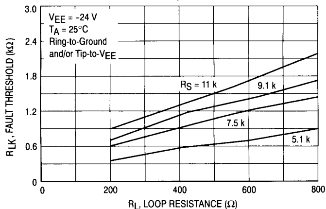
Figure 14. Fault Threshold (Off-Hook) versus Loop Resistance
