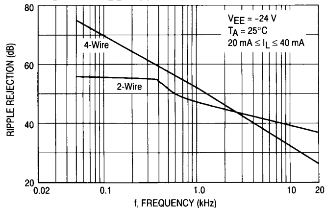
Figure 16. V_{DD} Ripple Rejection versus Frequency
