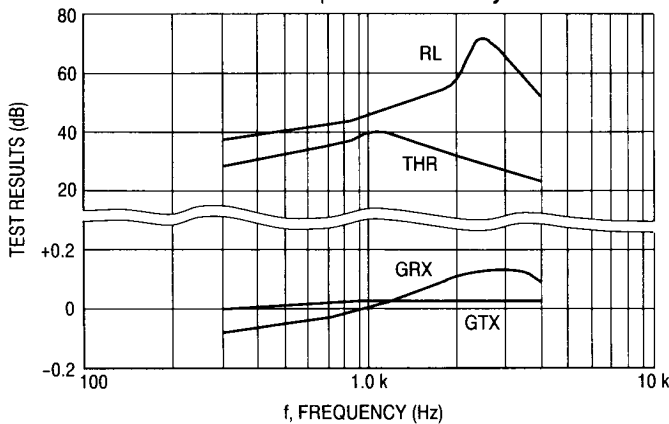
Figure 51. Circuit Performance 820 \Omega /0.115 \mu F and 220 \Omega System
