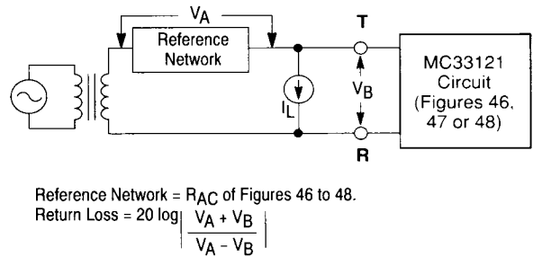
Figure 52. Return Loss Test Circuit for Figures 46 to 51
