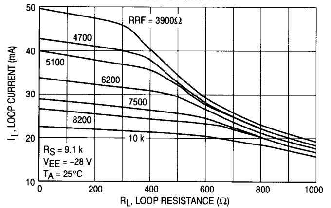
Figure 6. Loop Current versus Loop Resistance and RRF
