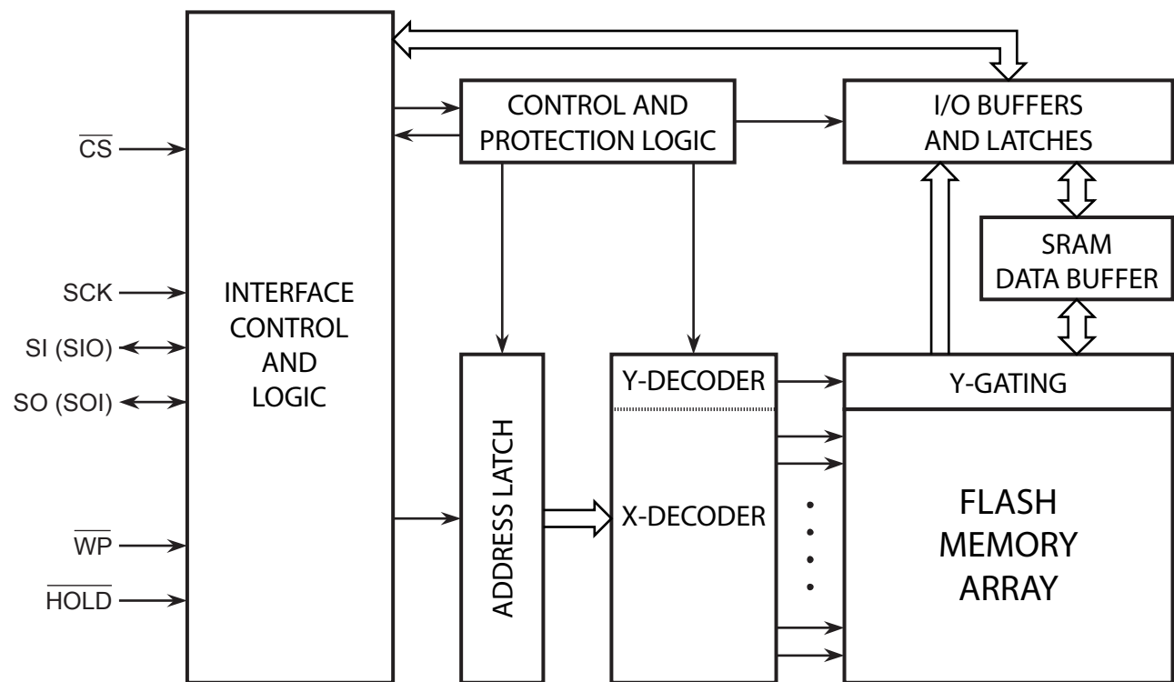
Figure 2-1. Block Diagram
