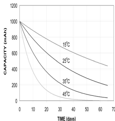
Figure 7. Self-Discharge at 2.5%/Day @ 25^\circ\text{C}
