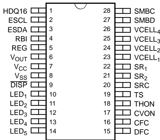
28-pin 150-mil SSOP
