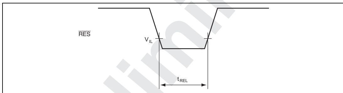
Figure 25.3 \overline{RES} Low Width Timing
