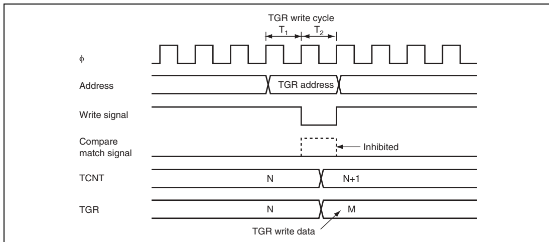
Figure 12.34 Contention between TGR Write and Compare Match
