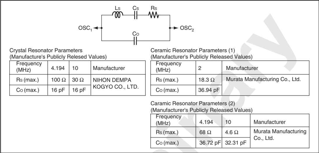
Figure 25.10 Resonator Equivalent Circuit
