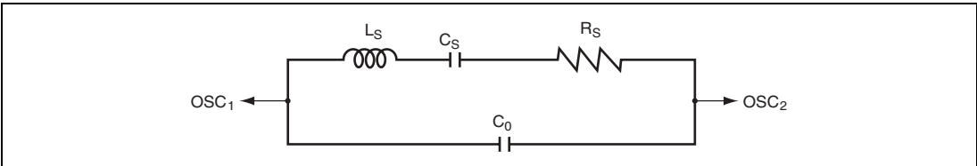
Figure 5.3 Equivalent Circuit of Crystal Resonator
