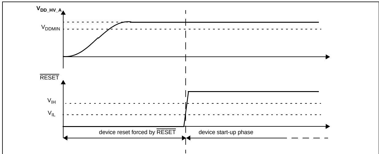
Figure 6. Start-up reset requirements
