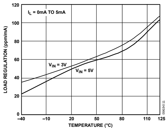
Figure 10. ADR390 Load Regulation vs. Temperature
