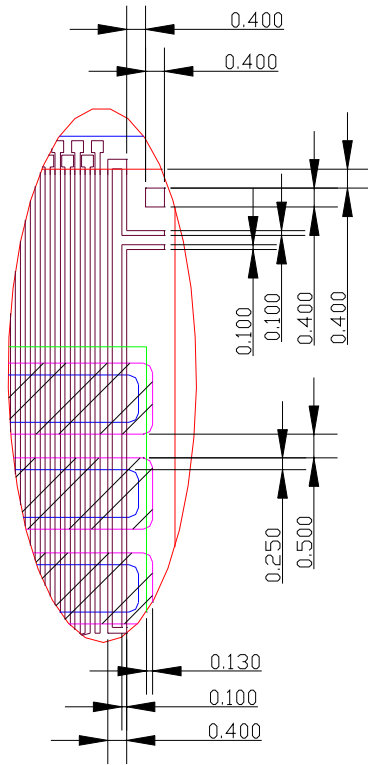
DETAIL A
