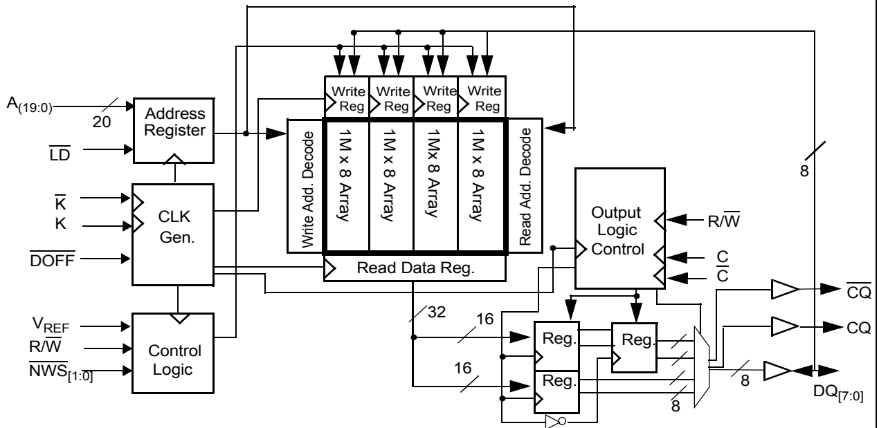
Logic Block Diagram (CY7C1417AV18)
