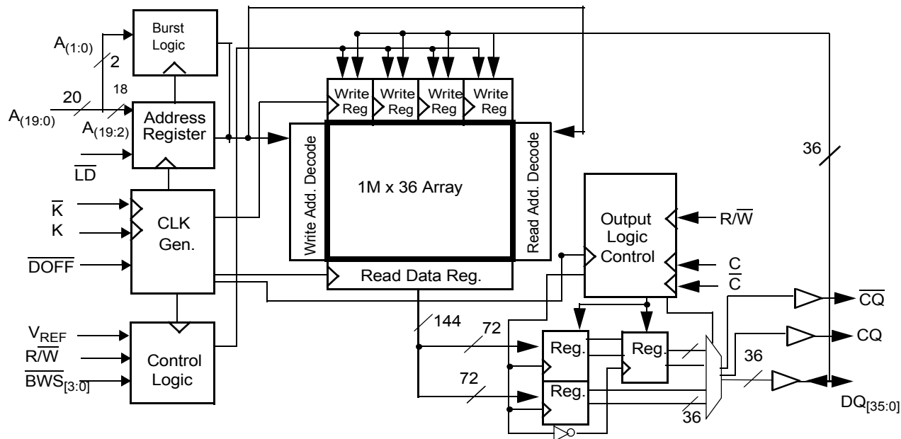
Logic Block Diagram (CY7C1421AV18)
