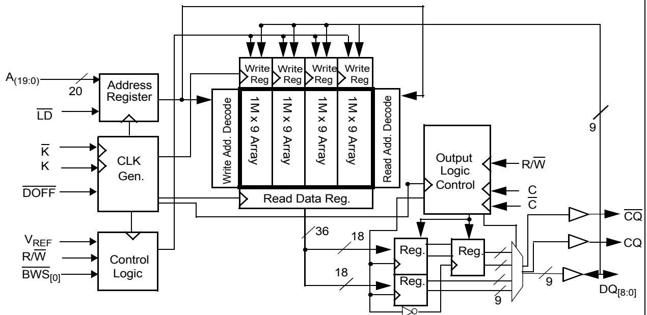
Logic Block Diagram (CY7C1428AV18)
