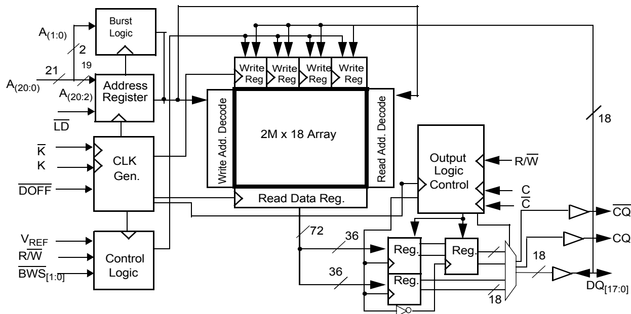
Logic Block Diagram (CY7C1419AV18)
