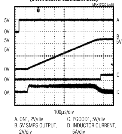
STARTUP WAVEFORMS (SWITCHING REGULATORS)
