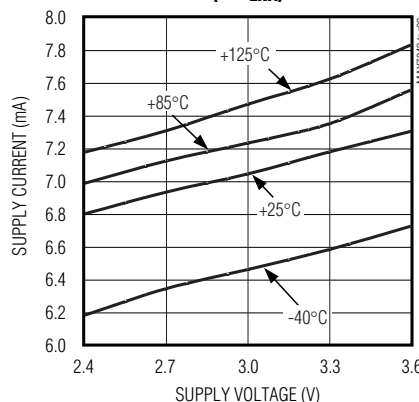
SUPPLY CURRENT vs. SUPPLY VOLTAGE (2x I_{LNA} )
