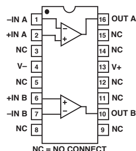
16-Pin SOL (S-Suffix)
