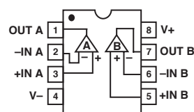
Epoxy Mini-DIP (P-Suffix) 8-Pin Hermetic DIP (Z-Suffix)
