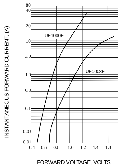
Fig. 5-TYPICAL FORWARD CHARACTERISTICS
