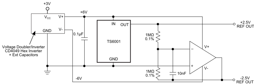
Figure 8: Generating Positive and Negative 2.5V References from a Single +3\text{V} or +5\text{V} Supply.
