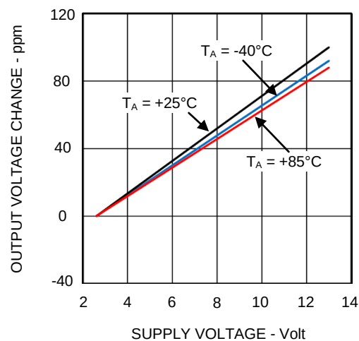
Line Regulation
