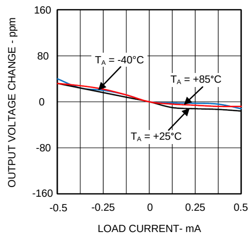
Load Regulation
