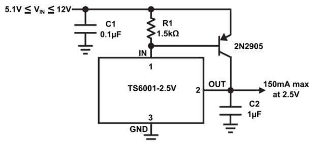
Figure 7: Boosting the TS6001's Output Current with an External PNP Transistor.
