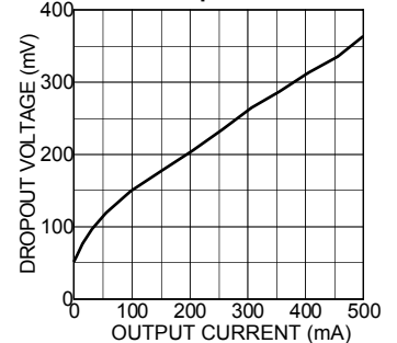
Dropout Voltage vs. Output Current
