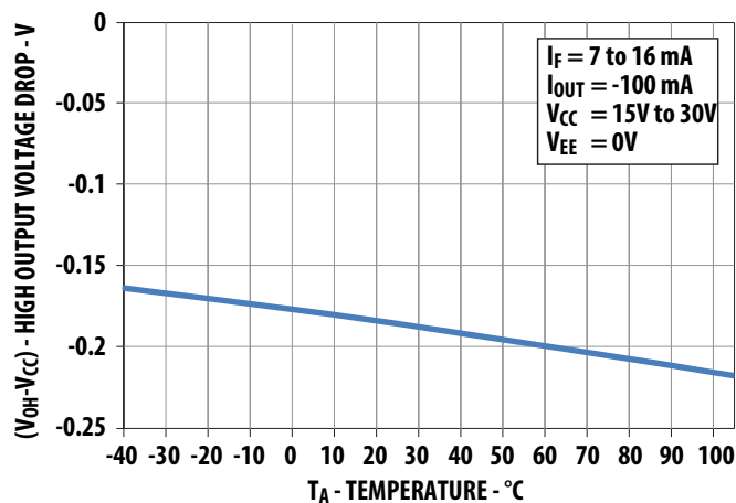
Figure 2 V_{OH} vs. Temperature
