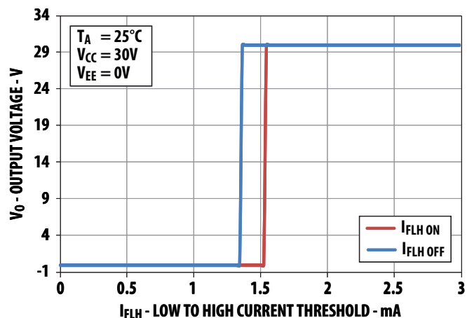
Figure 6 I_{FLH} Hysteresis
