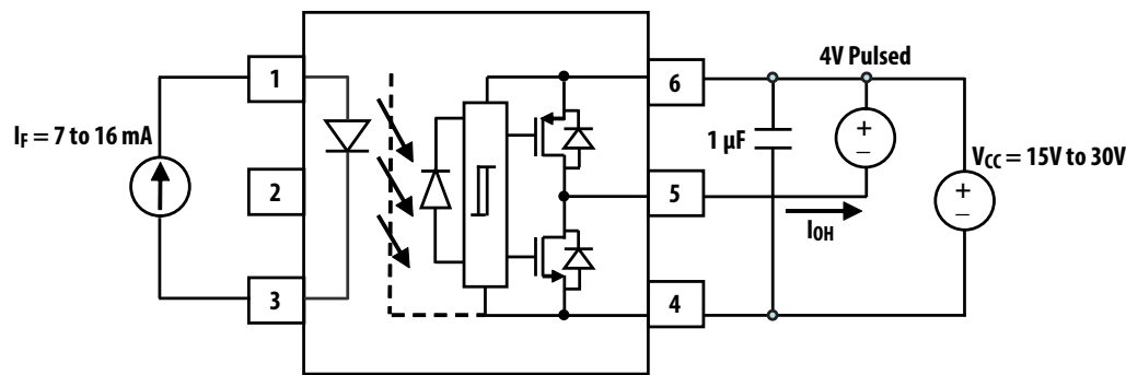
Figure 14 I_{OH} Test Circuit
