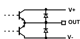
CIRCUIT 3
