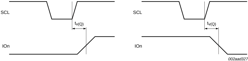
Fig 22. t_{v(Q)} timing
