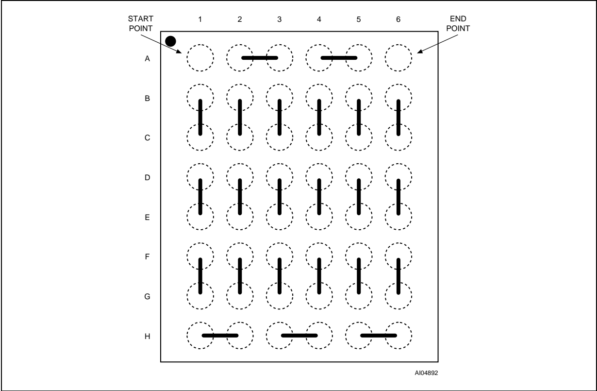
Figure 17. TFBGA48 Daisy Chain - PCB Connections (Top view through package)
