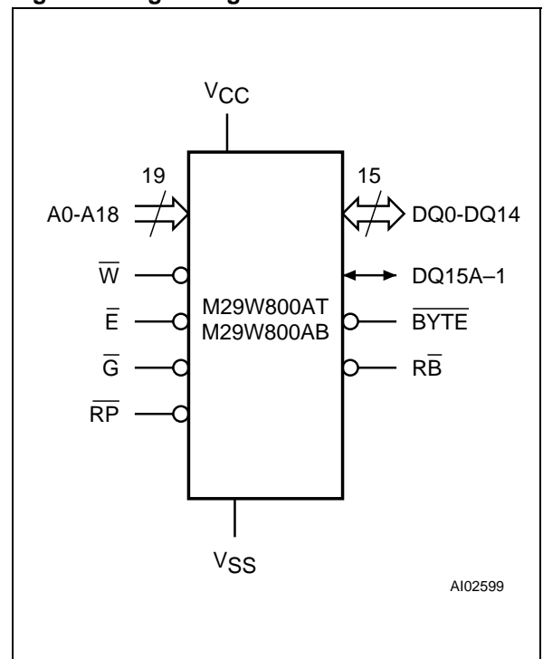
Figure 1. Logic Diagram
