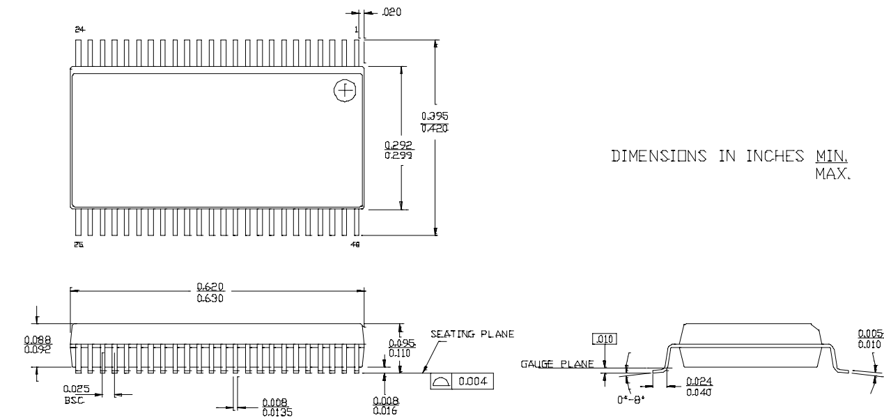
Figure 2-6. 48-Lead (300-Mil) SSOP
