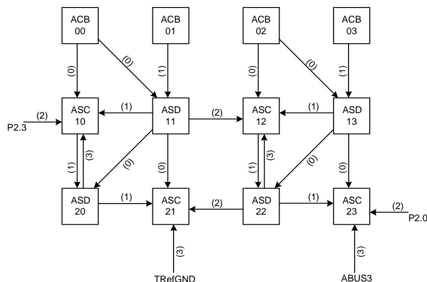
Figure 19-6. BMuxSC/SD Connections
