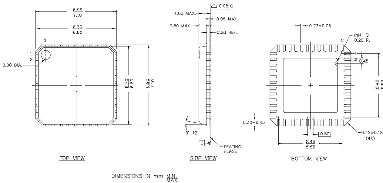
Figure 2-7. 48-Lead (7x7 mm) MLF
