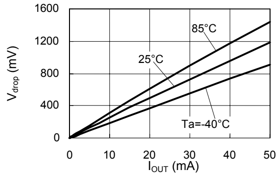
S-817A30A/S-817B30A
