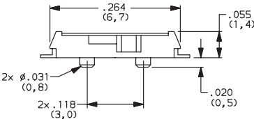
PCM12SMTR SPDT
