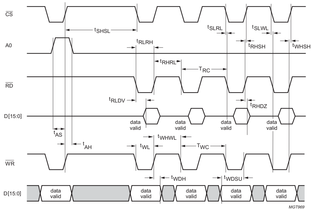
Fig 49. HC Programmed interface timing.
