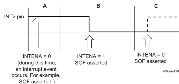
Fig 22. Behavior of bit INTENA .
