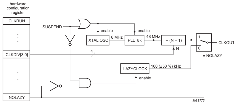
Fig 47. Oscillator and LazyClock logic.
