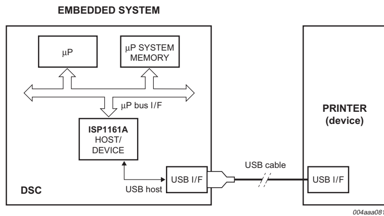
Fig 2. ISP1161A operating as a stand-alone USB host.
