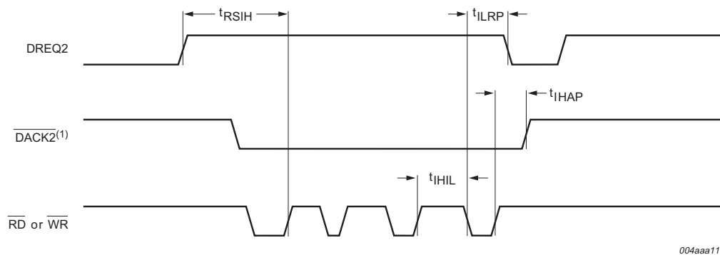
Fig 60. DC burst mode DMA timing.
