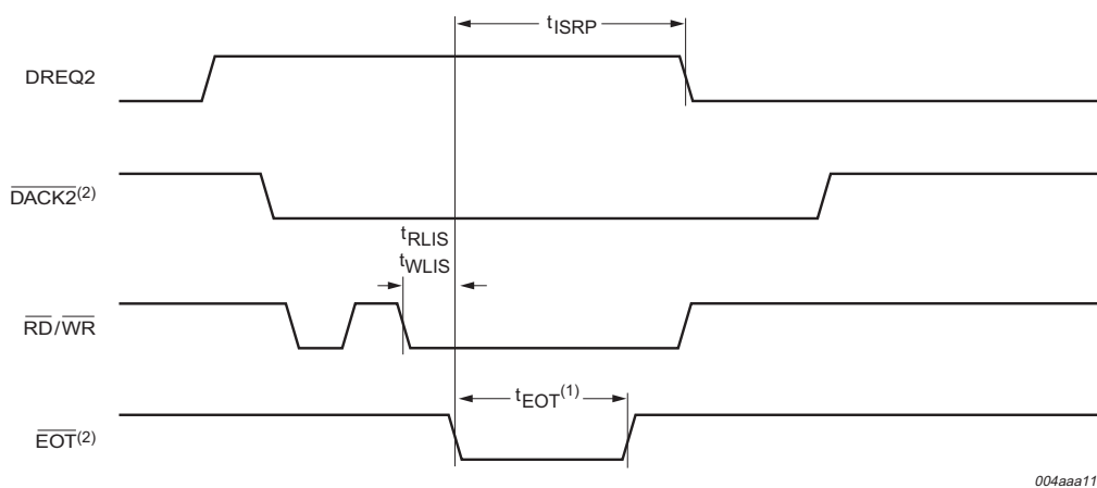
Fig 61. EOT timing in DC burst mode DMA.
