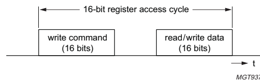
Fig 12. 16-bit register access cycle.
