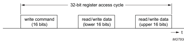
Fig 13. 32-bit register access cycle.
