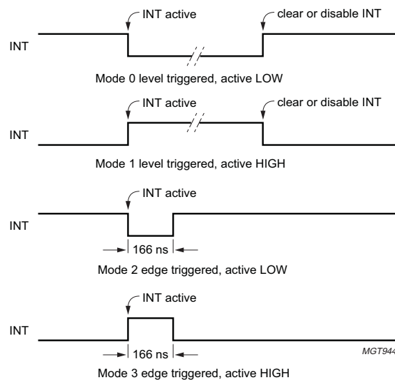
Fig 19. Interrupt pin operating modes.
