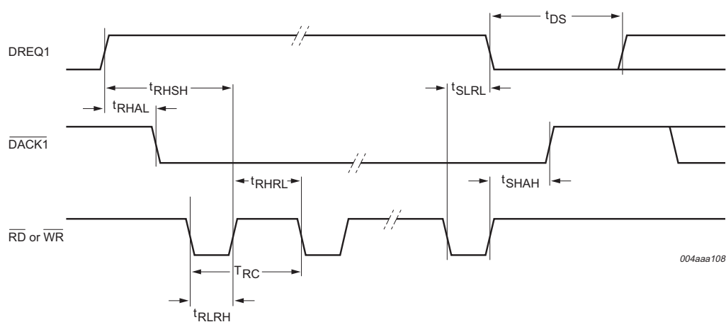
Fig 53. HC burst mode DMA timing.
