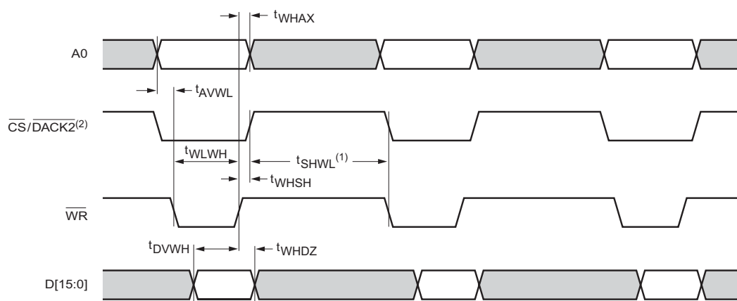
Fig 50. DC Programmed interface read timing (I/O and 8237 compatible DMA).
