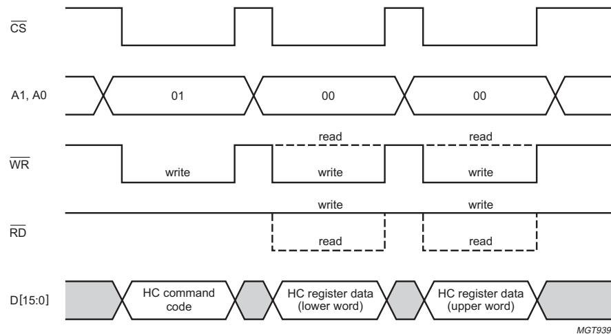
Fig 14. Accessing HC control registers.
