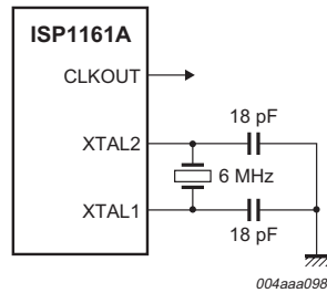
Fig 45. Oscillator circuit with external crystal.
