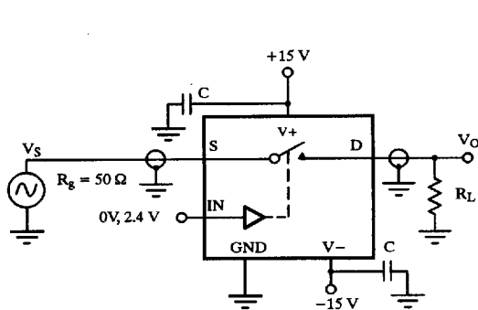
Figure 3. Charge Injection
