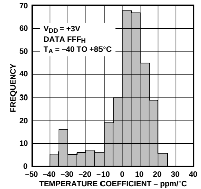
Figure 19. Full-Scale Output Tempco Histogram
