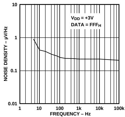
Figure 16. Output Voltage Noise Density vs. Frequency
