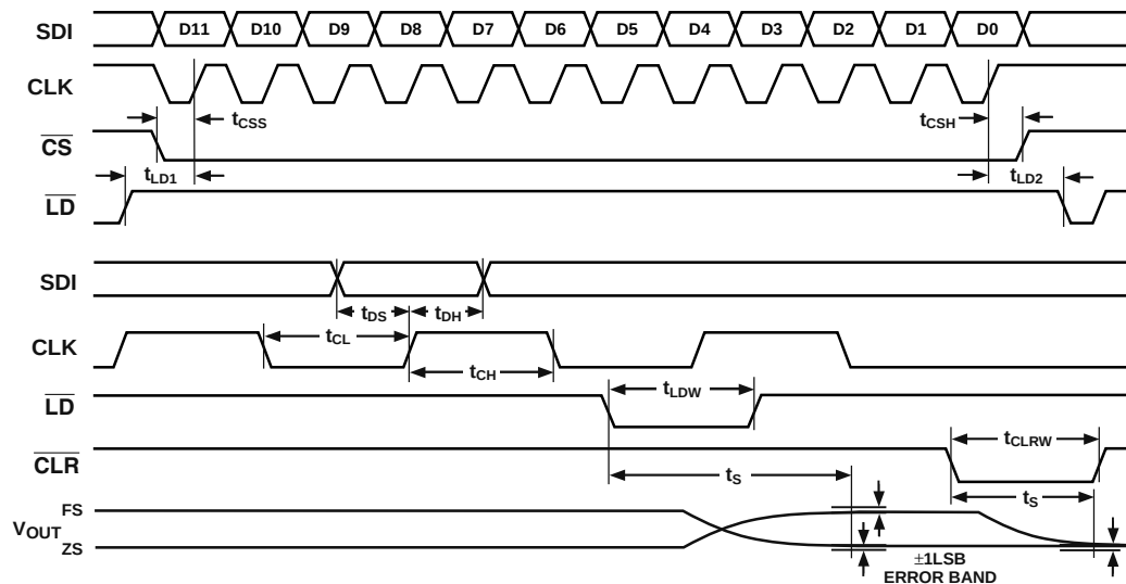
Figure 3. Timing Diagram
