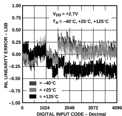
Figure 2. Linearity Error vs. Digital Code and Temperature
