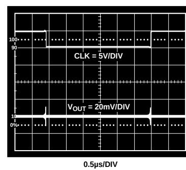
Figure 12. Digital Feedthrough vs. Time
