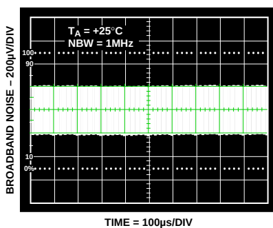
Figure 5. Broadband Noise
