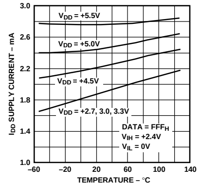
Figure 18. Supply Current vs. Temperature
