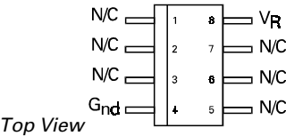
SO8 Package Suffix – N8
