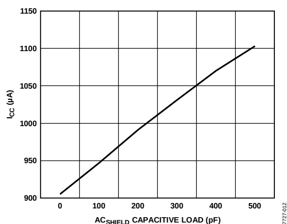
Figure 12. Supply Current vs. Capacitive Load on AC_SHEILD
