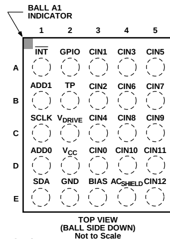
Figure 6. AD7147A-1 Pin Configuration
