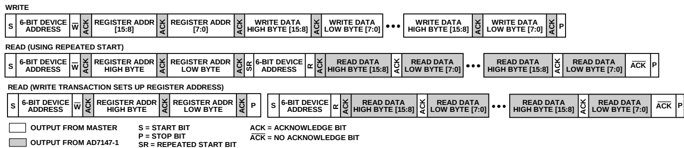
Figure 54. Example of Sequential I²C Write and Readback Operations
