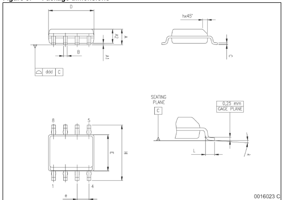
Figure 9. Package dimensions
