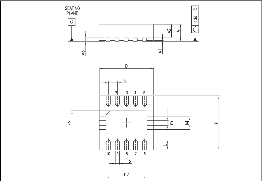
Figure 10. Package dimensions
