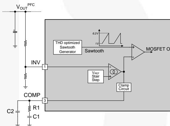
Figure 31. Control Circuit
