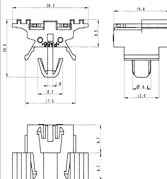
Fixing clip - AB02SFT
