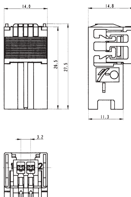
Male housing
