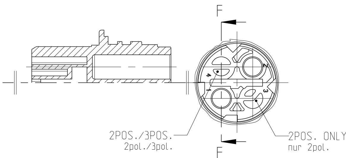
CLOSED CAVITIES OF THE 2POS./3POS. SOCKET HOUSING Geschlossene Kammern des 2pol./3pol. Buchsengehaeuses
