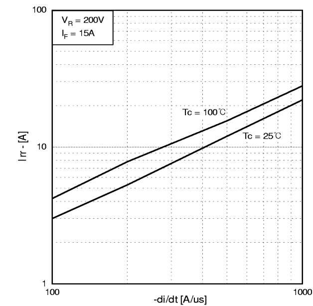
Fig.14 Typical Reverse Recovery Current vs. di/dt
