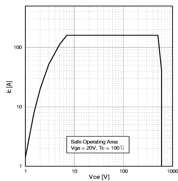
Fig.11 Turn-off SOA
