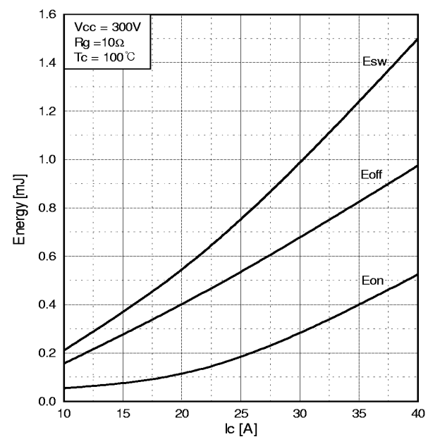
Fig.10 Typical Switching loss vs. Collector to Emitter Current
