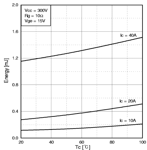
Fig.9 Typical Switching Loss vs. Case Temperature
