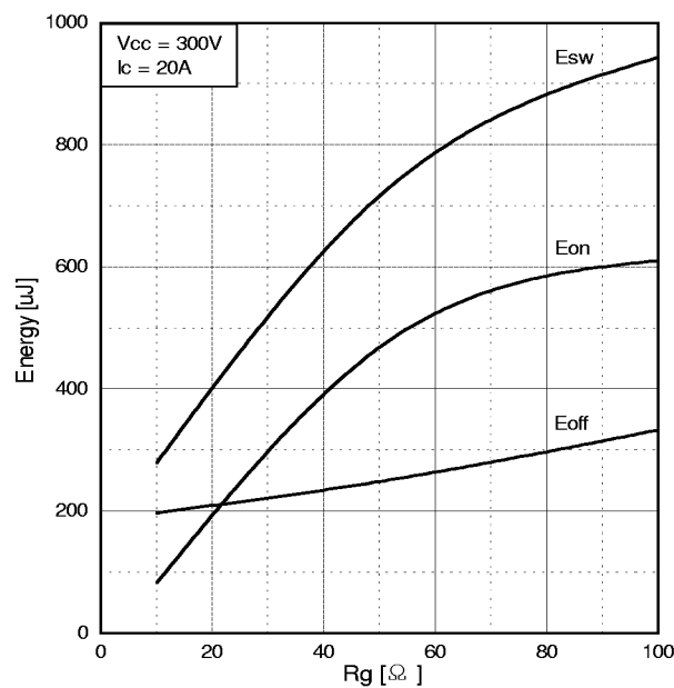
Fig.8 Typical Switching Loss vs. Gate Resistance
