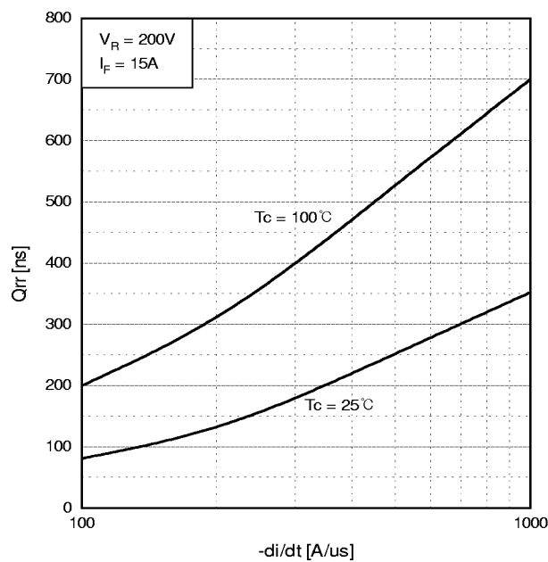
Fig.15 Typical Stored Charge vs. di/dt
