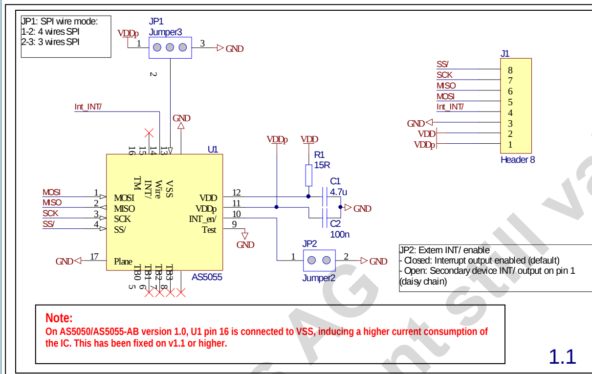
Figure 4: AS5050-AB-1.1 adapterboard schematics
