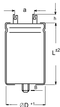
Fig 2: Version LFB for stud mounting
