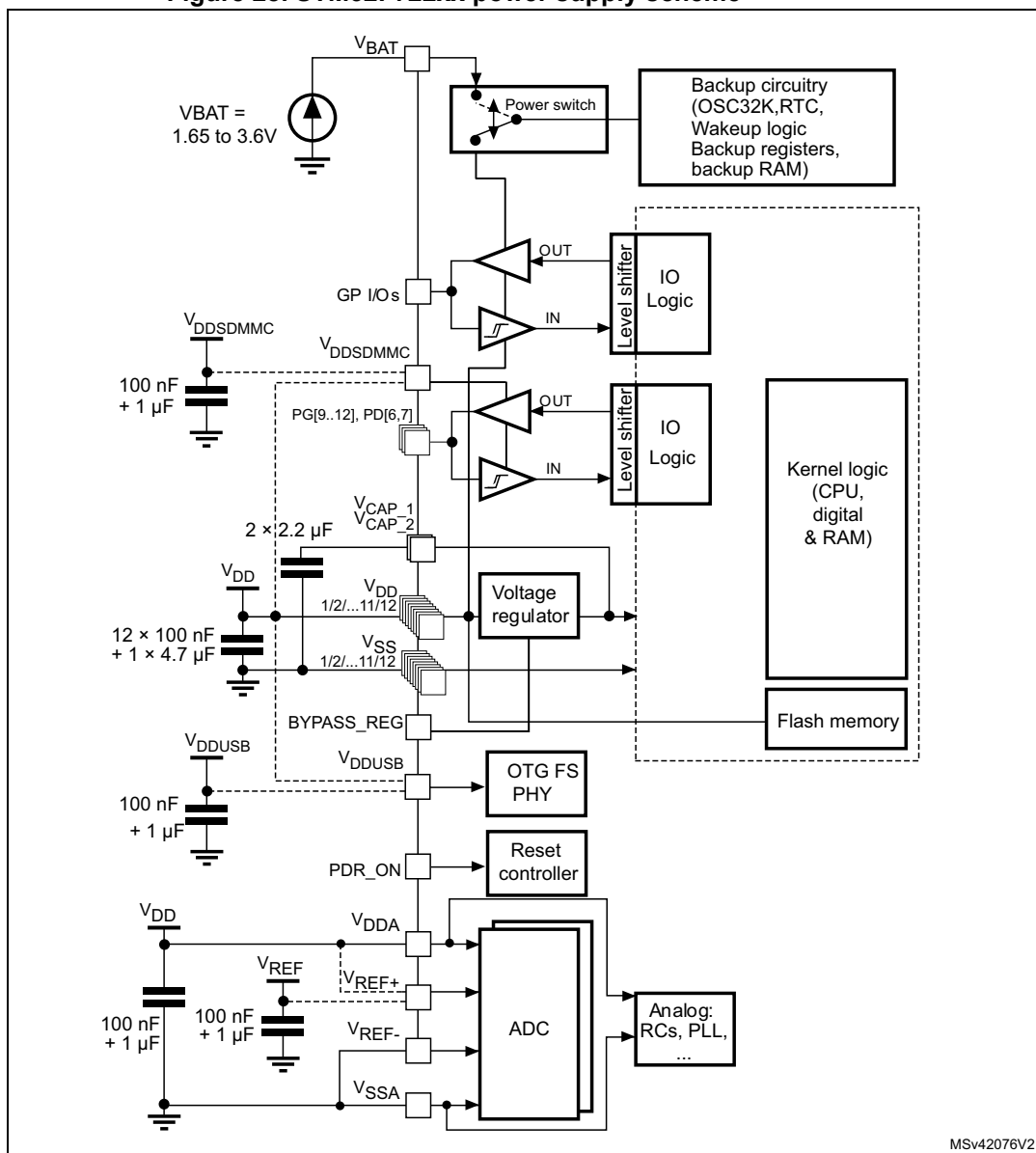
Figure 28. STM32F722xx power supply scheme
