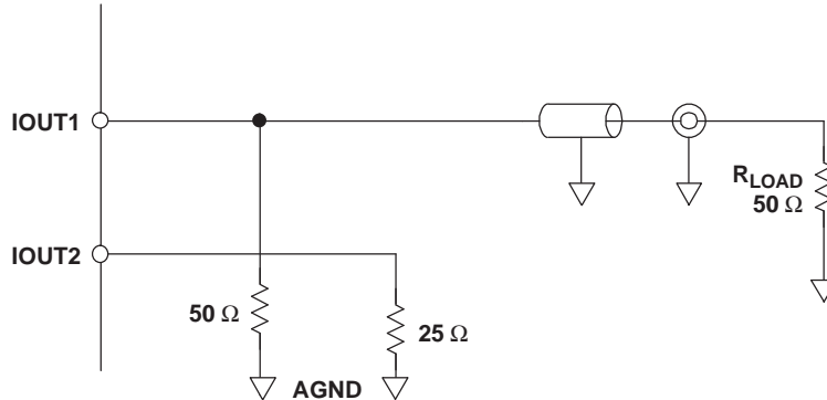
Figure 20. Driving a Doubly-Terminated 50-Ω Cable Using a Single-Ended Output
