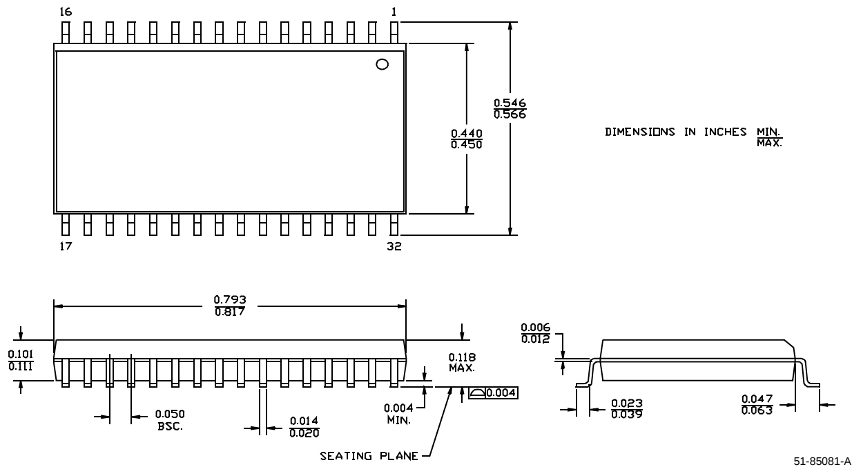
32-lead (450-mil) Molded SOIC S34
