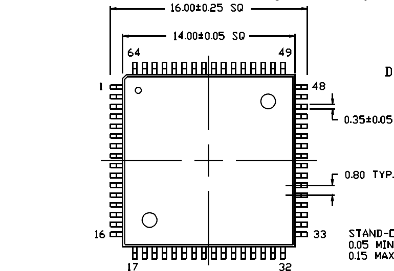
64-lead Thin Plastic Quad Flat Pack (14 × 14 × 1.4 mm) A65
