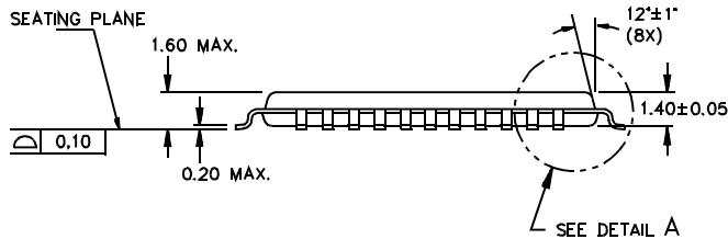
64-lead Thin Plastic Quad Flat Pack (14 × 14 × 1.4 mm) A65
