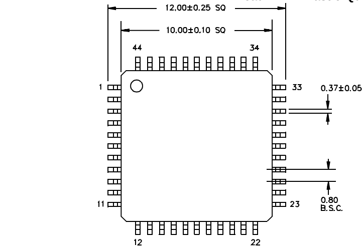
44-lead Thin Plastic Quad Flat Pack A44
