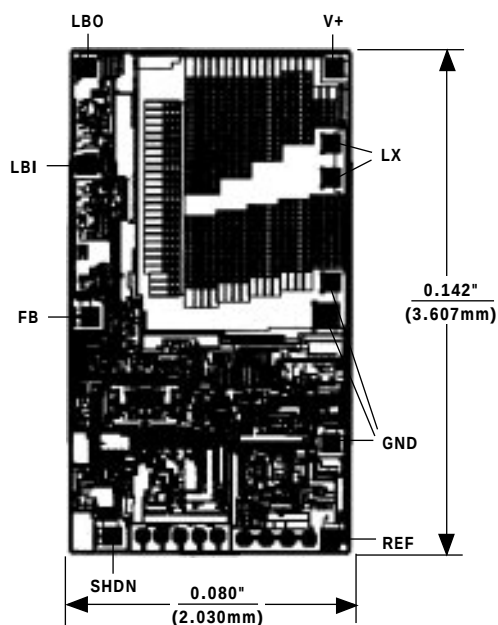
Chip Topography
