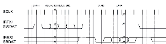
Figure 20. Read Data Waveform
