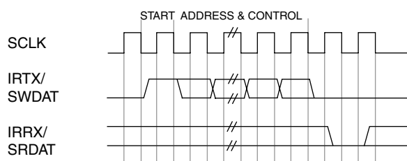
Figure 16. Special Command Waveform
