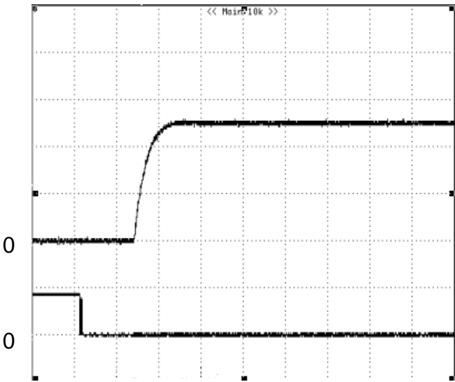
Figure 5: Turn-on transient at zero load current (1 ms/div). Vin=48V. Top Trace: Vout, 1.0V/div; Bottom Trace: ON/OFF input, 5V/div
