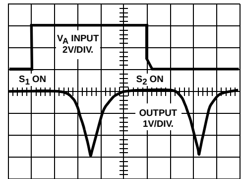
FIGURE 2C. WAVEFORMS
