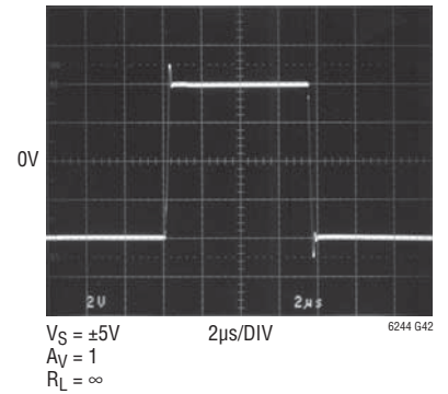
Large-Signal Response
