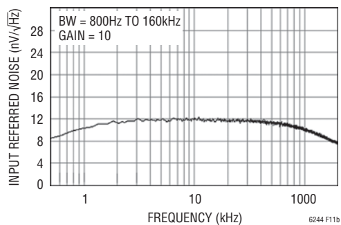
Figure 11b. Input Referred Noise
